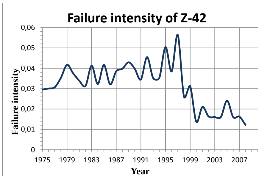
Fig. 2: Failure intensity of the aircraft ZLIN Z-42
